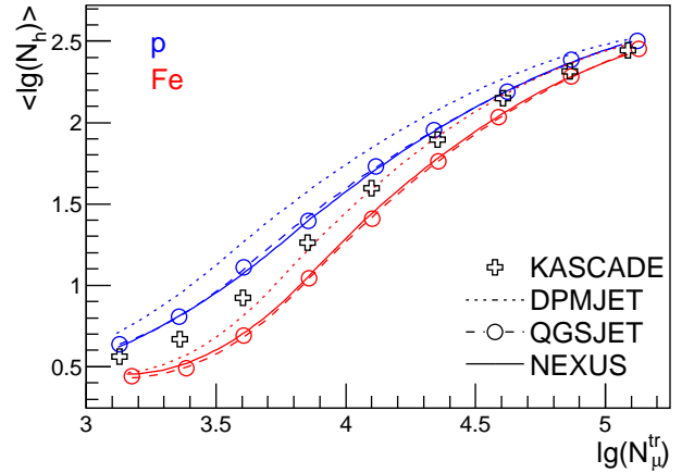
Fig. 1. Hadron number N_h versus muon number N_\mu^{\text{tr}} .
