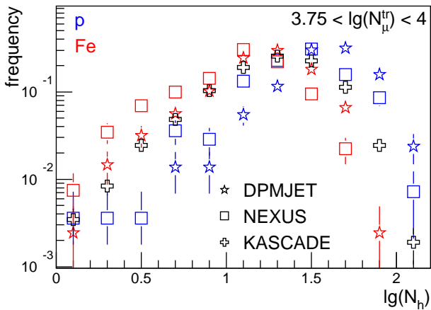
Fig. 3. Frequency distribution of the hadron number N_h . The muon number bin corresponds to a primary energy of about 2 PeV. The QGSJET distributions, not plotted here, are similar to NEXUS.
