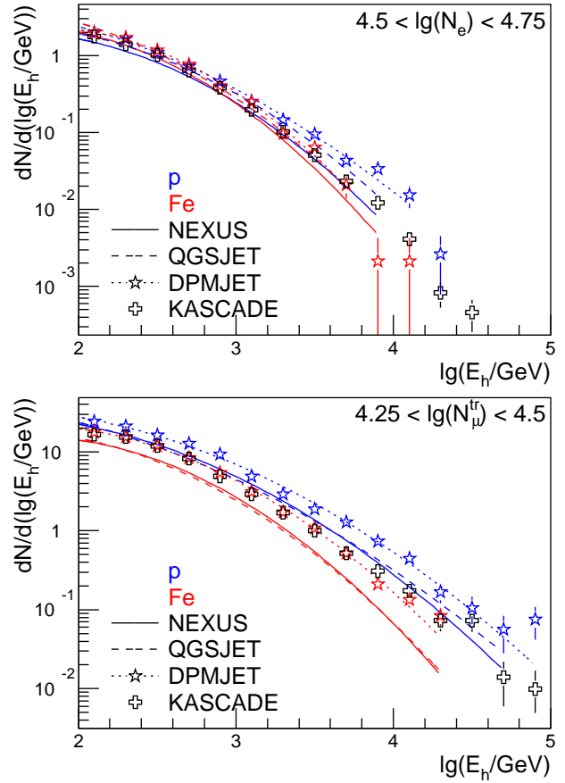
Fig. 7. Energy spectra of hadrons.
