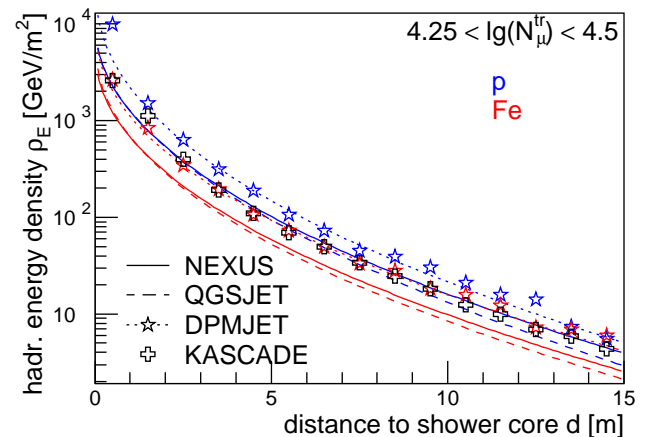
Fig. 5. Lateral distribution of the hadronic energy density. The muon number bin corresponds to a primary energy of 8 PeV.
