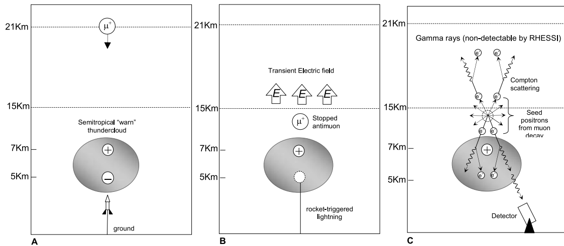
Figure 2. Mechanism for production of TGFs seen on the ground. (a) Small thunderclouds can stop positive muons by (b) rocket-triggered lightning. (c) It will produce gamma rays on the ground.
